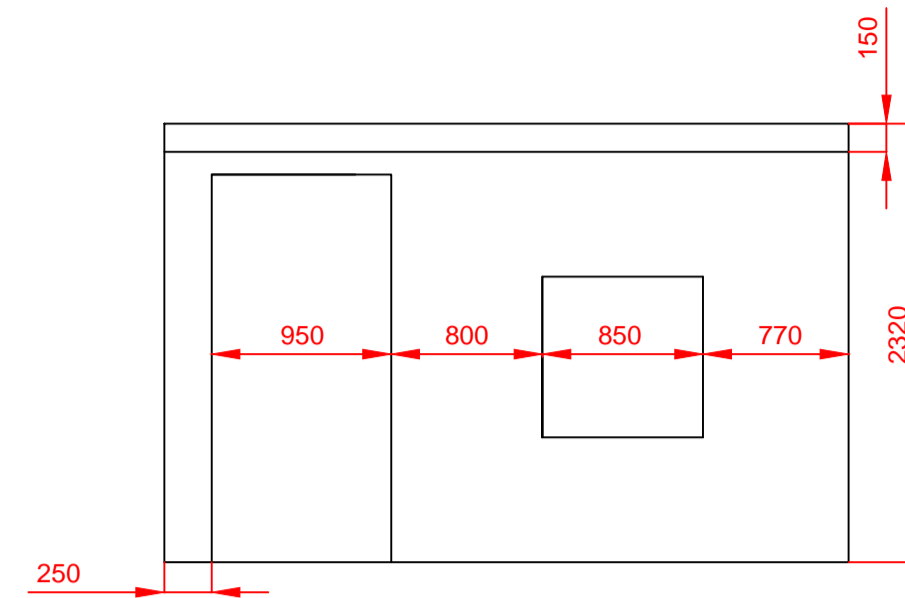
SECTION A-A ELEVATION
